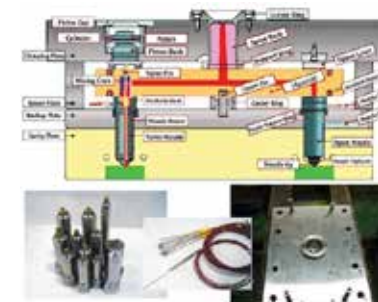
Hot Runner System(HRS)
